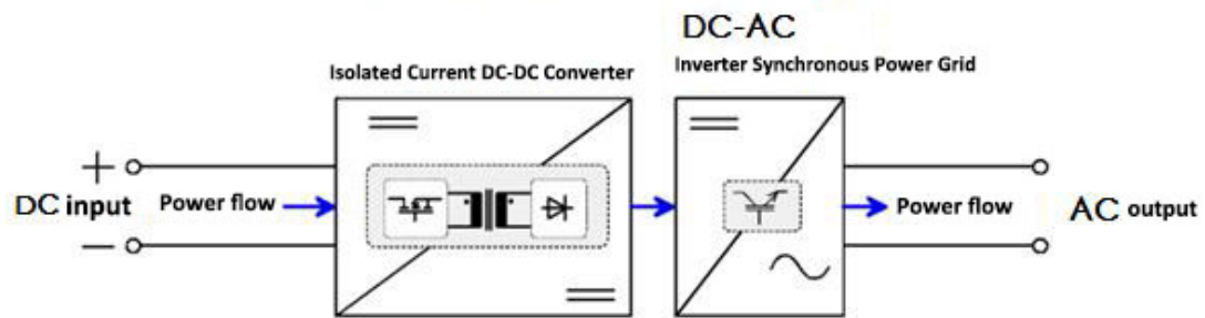
Figure 2: stages from IT8300 DC input to grid-tied inverter
