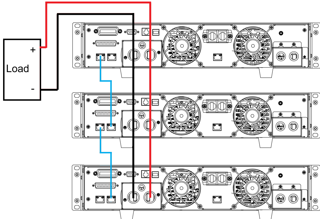
Figure 3–1 Schematic Diagram of 3 Pcs Power Supplies in Parallel
