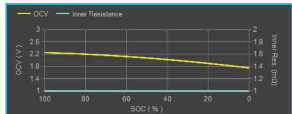
Lead-acid battery
