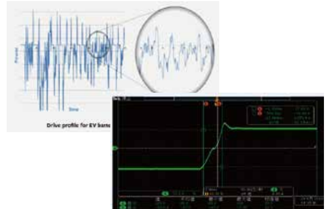
ITS5300 battery pack test system current switching waveform
